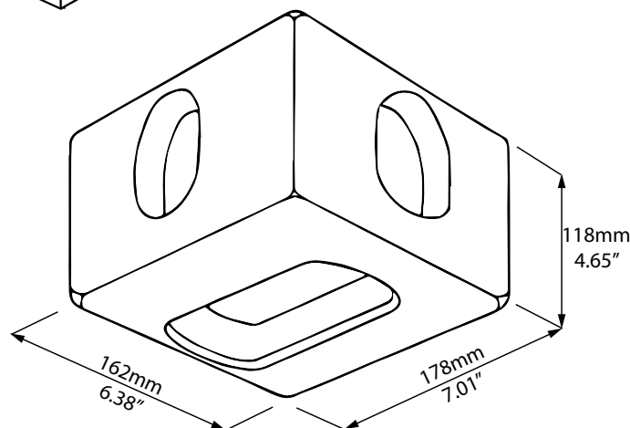
Bottom Left Corner Casting Bottom Right Corner Casting (Symmetrical)
